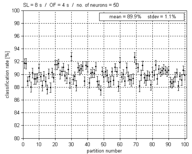
Figure 5: Classification rates of 100 fixed training set / test set partitions and different initializations. Grand mean and standard deviation of mean classification rates was computed.
