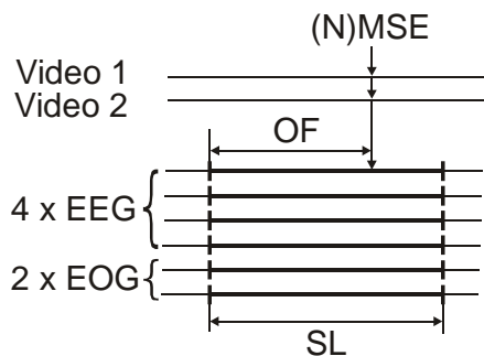
Figure 1: Segmentation of EEG- / EOG- signals with relation to visually scored microsleep- (MSE) or nonmicrosleep- (NMSE) events by two parameters offset (OF) and segment length (SL).
